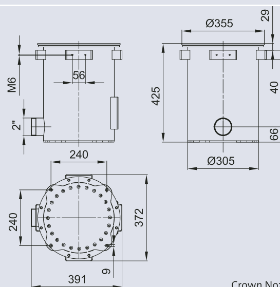
Crown Nozzle
