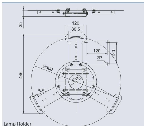
Lamp Holder
