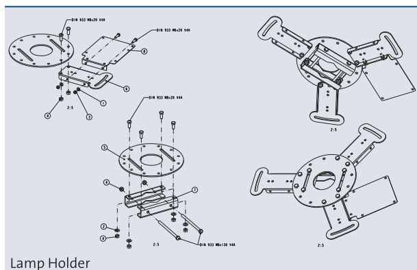
Lamp Holder
