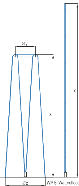
WP4: Watereffect Screen Jet high WP5: Watereffect High Jet
